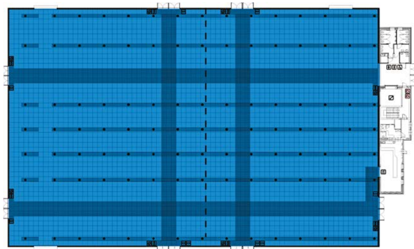
Hall 3 - floorplan
